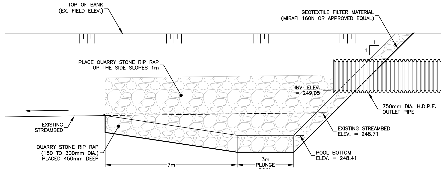
TYPICAL PLUNGE POOL DETAIL
