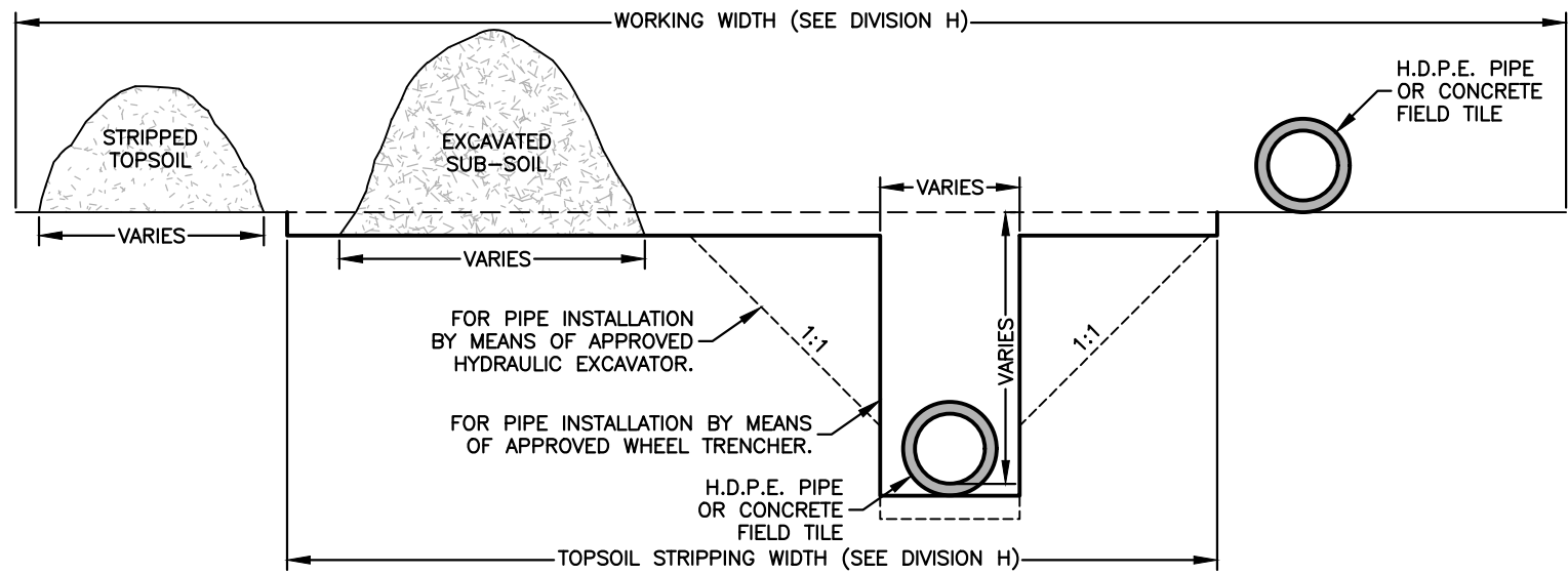
TYPICAL WORKING CORRIDOR DETAIL
