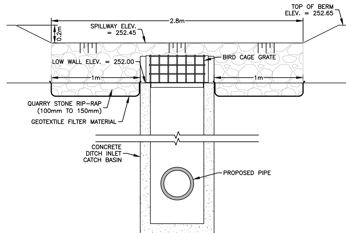
D.I.C.B. AND BERM (STA. 0+593) INSTALLATION DETAIL
