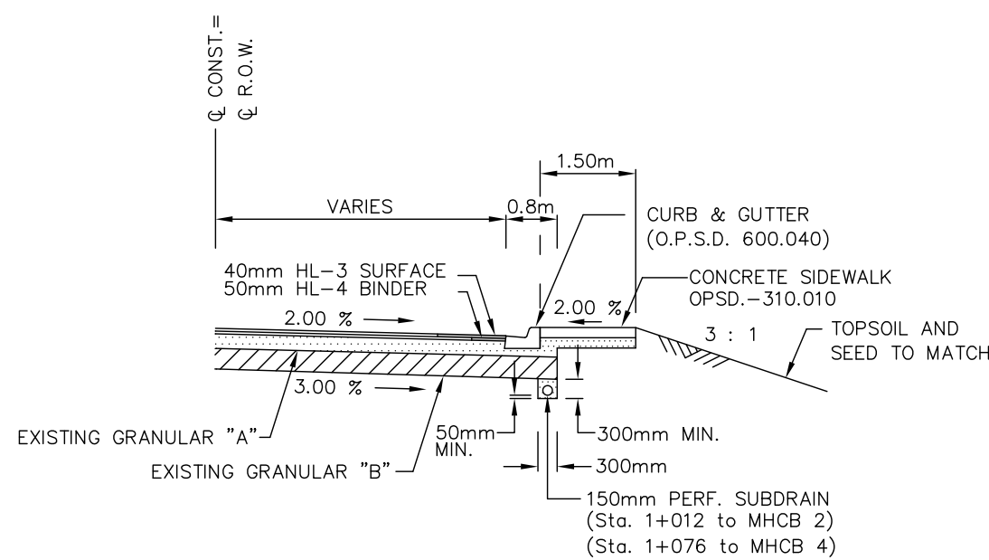
TYPICAL SECTION YOUNG STREET TO STA. 1+110 N.T.S.
