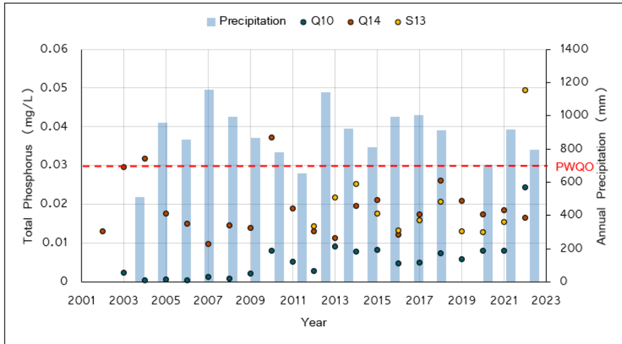
Figure 7: Annual average phosphorus concentrations (mg/L) for sampling locations within the South Saugeen River sub- watershed from 2002 to 2022. SVCA internal sampling program began at S13 in 2012, no prior data available. PWQO= 0.03 mg/L.
